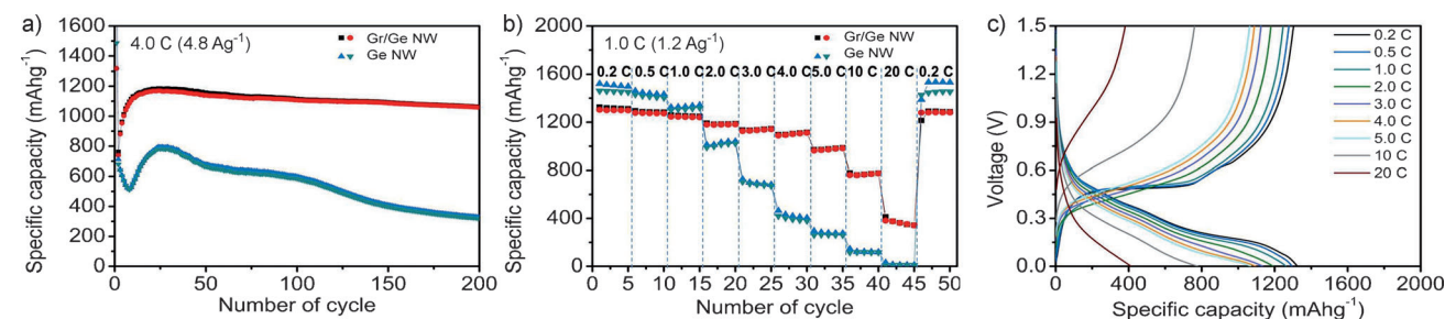
Figure 3. a) Comparison of the cycle performance of a Gr/Ge NW and a bare Ge NW at a rate of 4.0 C. b) Rate capability of a Gr/Ge NW and a bare Ge NW from 0.2 to 20 C. Legends: blue \blacktriangle charging of the Ge NW, green \blacktriangledown discharging of the Ge NW, black \blacksquare charging of the Gr/Ge NW, and red \bullet discharging of the Gr/Ge NW. c) Voltage profiles of the Gr/Ge NW corresponding to the rate capability measurement in (b).
